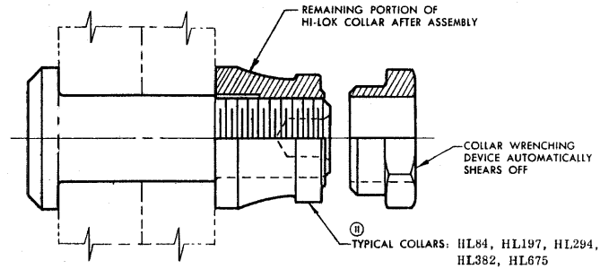
HI-LOK PIN AND COLLAR AFTER ASSEMBLY
